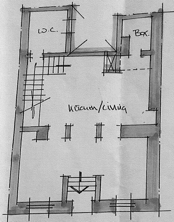
Ground Floor 1:100
