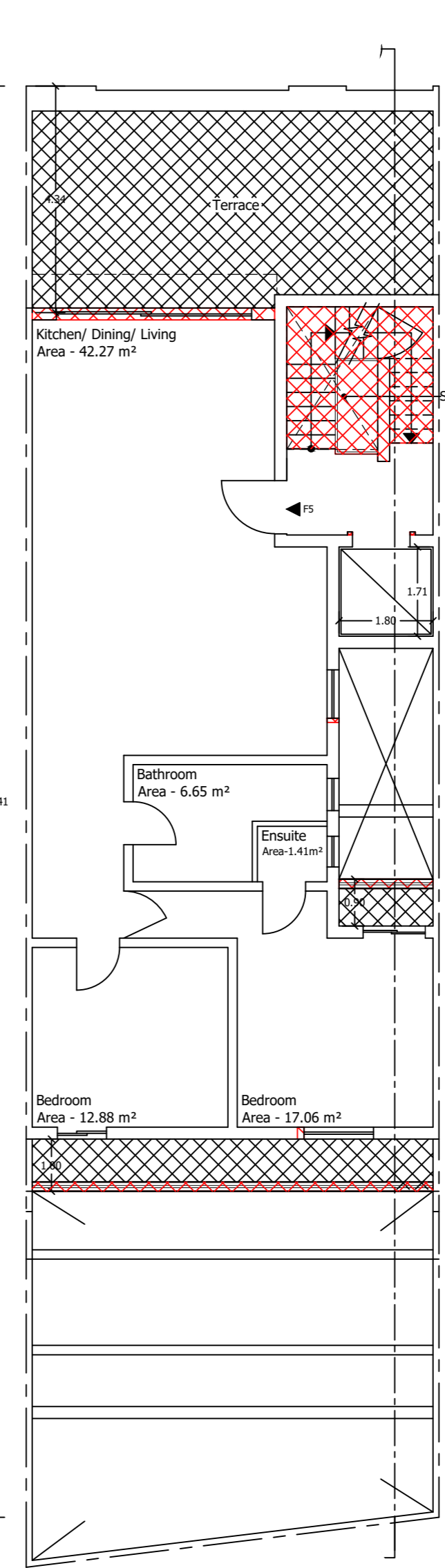
Proposed Setback Floor Scale 1:100
