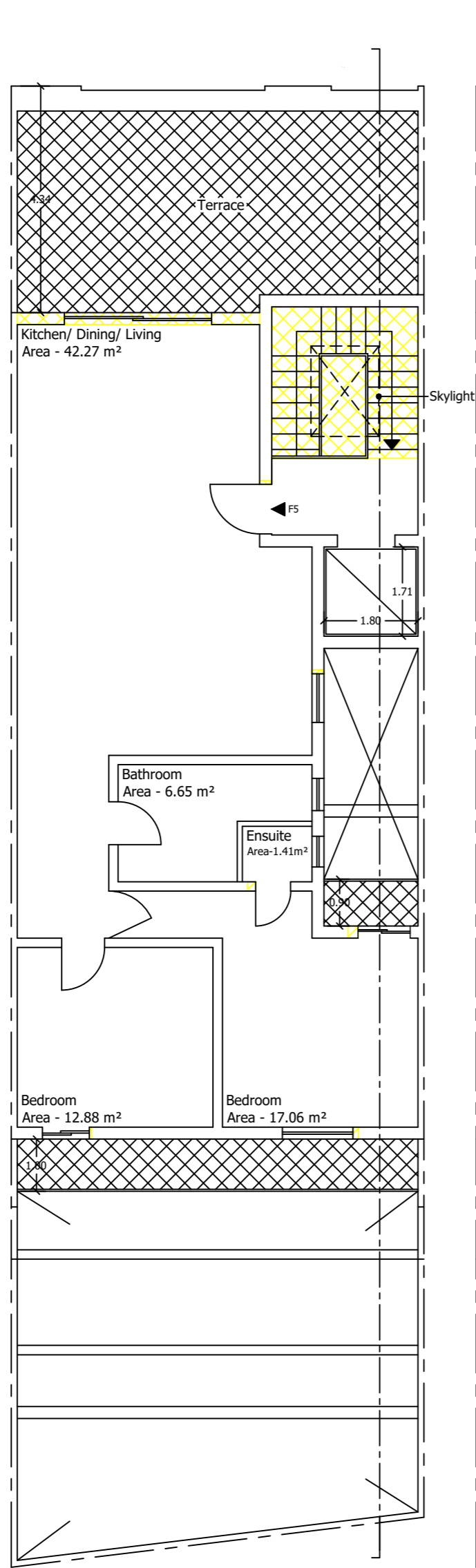
Approved Setback Floor Scale 1:100
