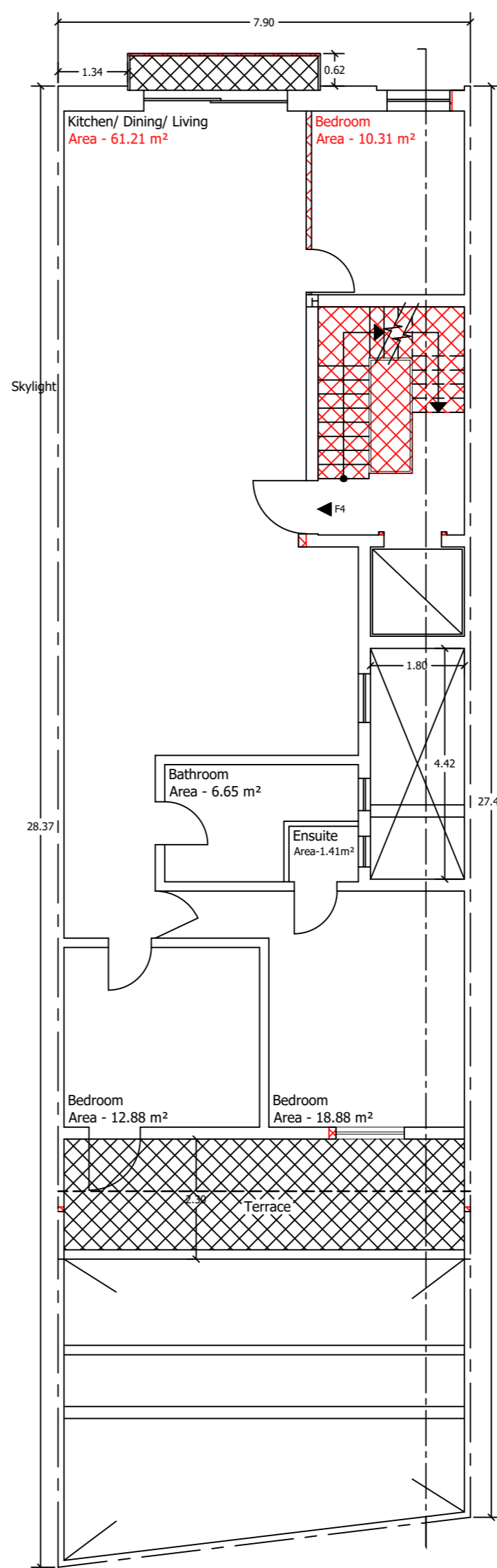
Proposed Fourth Floor Scale 1:100
