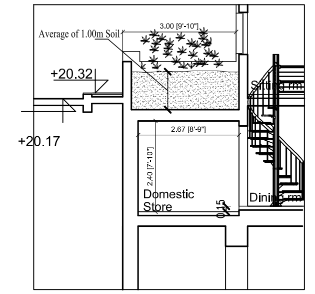
Section CC As Proposed Scale 1:100
