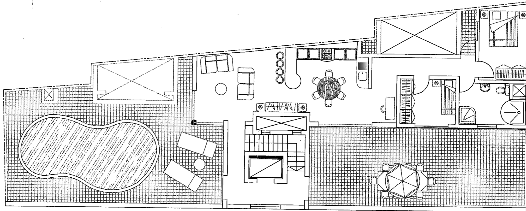
penthouse (1) 1:100
