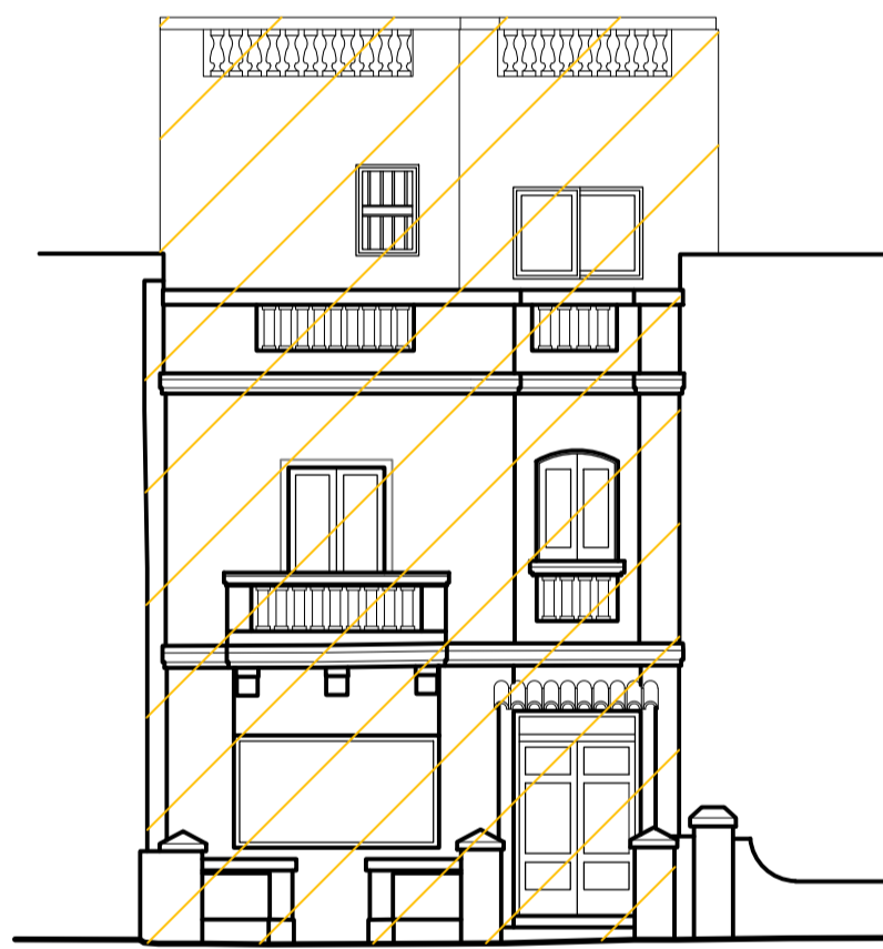
Existing Elevation Triq Bufula Hamra Scale 1:100
