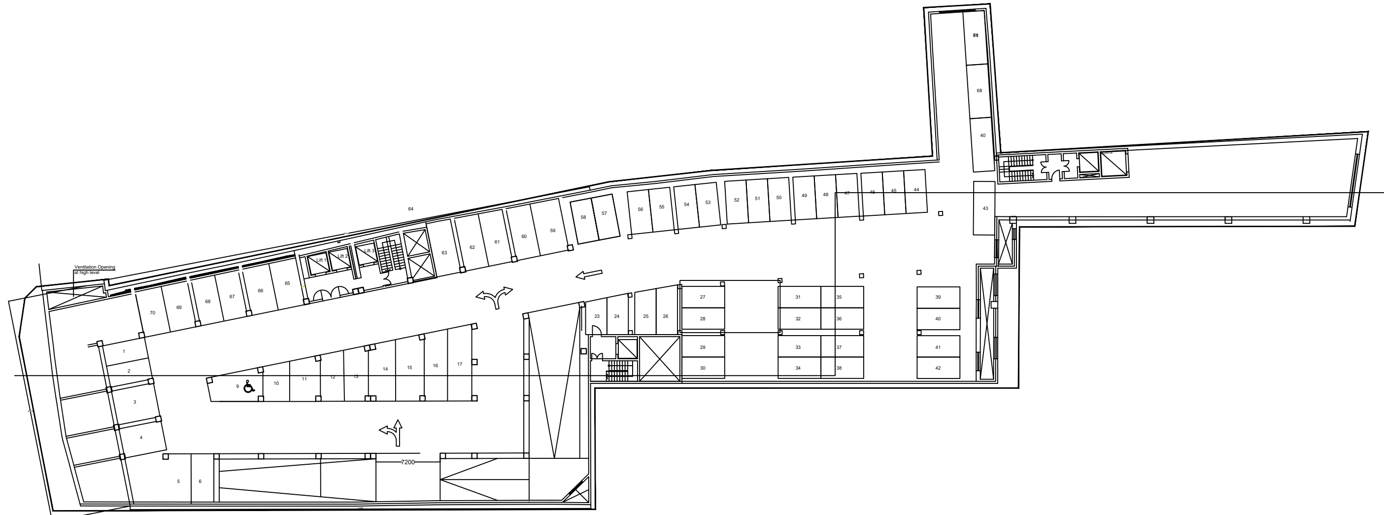
Architectural Layout - Basement level -1 Scale 1:200
