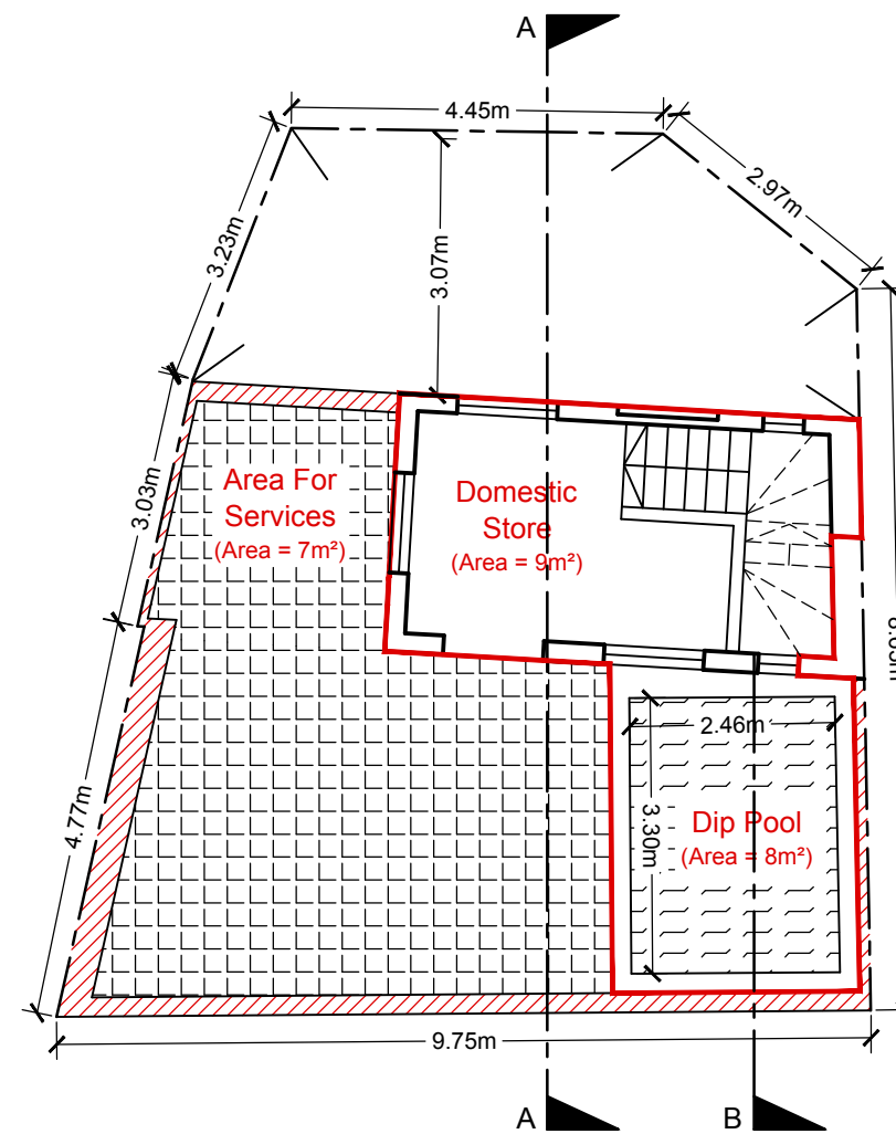
P6 PROPOSED SETBACK FLOOR PLAN D3 Floor Area = 65m 2 Scale 1:100
