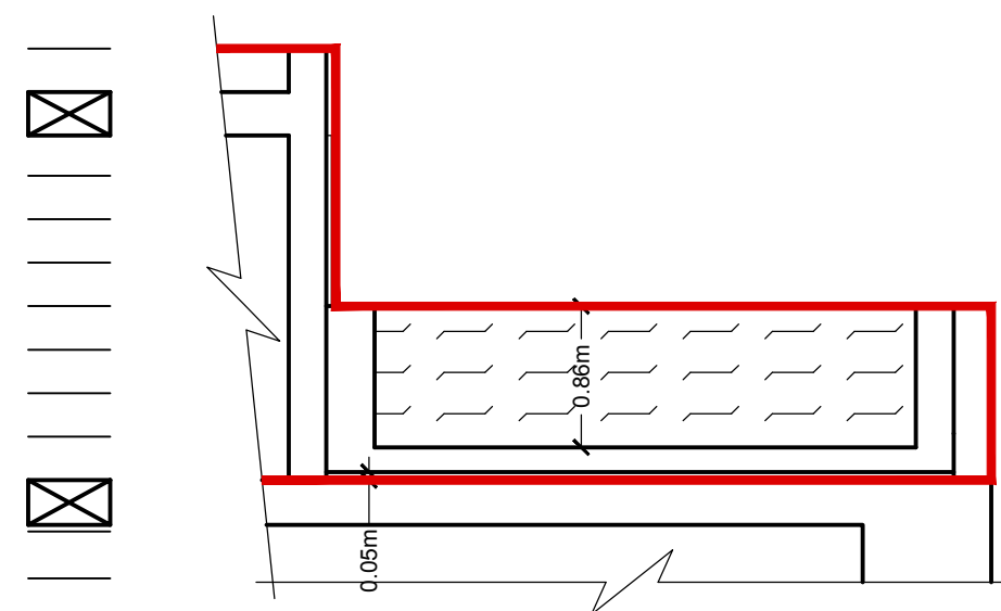
S3 PROPOSED SECTION B-B THROUGH DIP POOL D3 Scale 1:50
