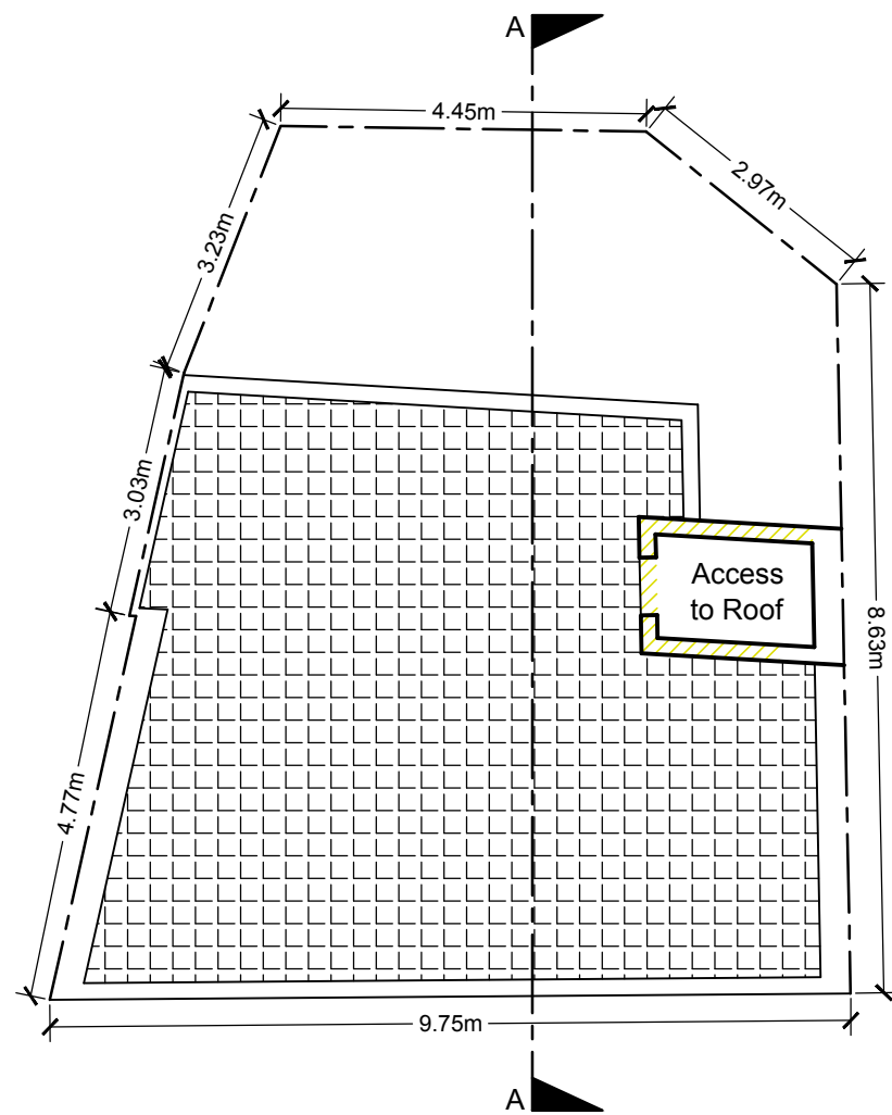
P5 EXISTING SETBACK FLOOR PLAN D3 Floor Area = 63m 2 Scale 1:100
