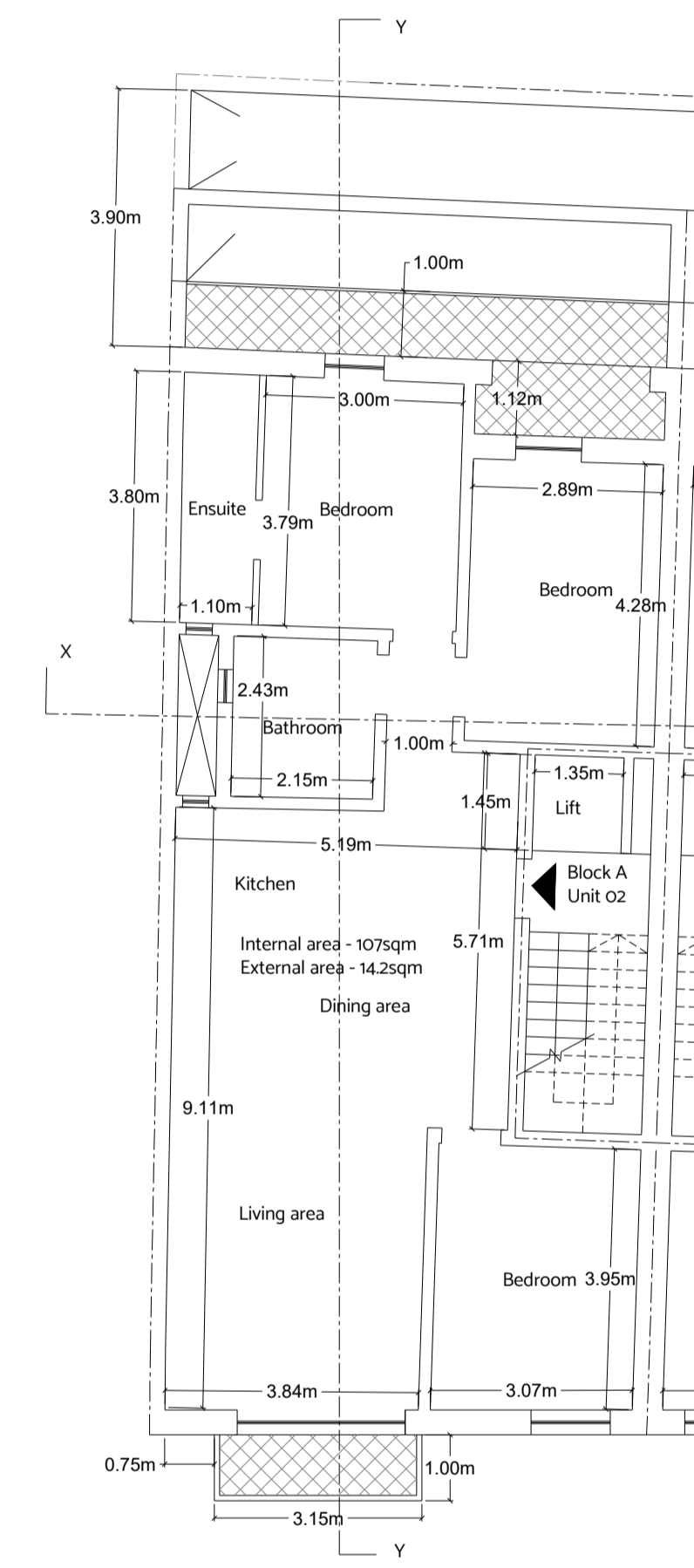
Approved Second Floor Level Plan Scale 1:100
