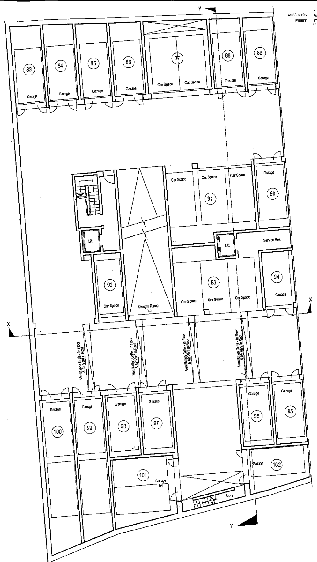
○ Proposed Level -5 Covered by PA 1349/11 Total Site Area - circa 2333.54 s.m. Total Built-Up Area - circa 1071 s.m.
