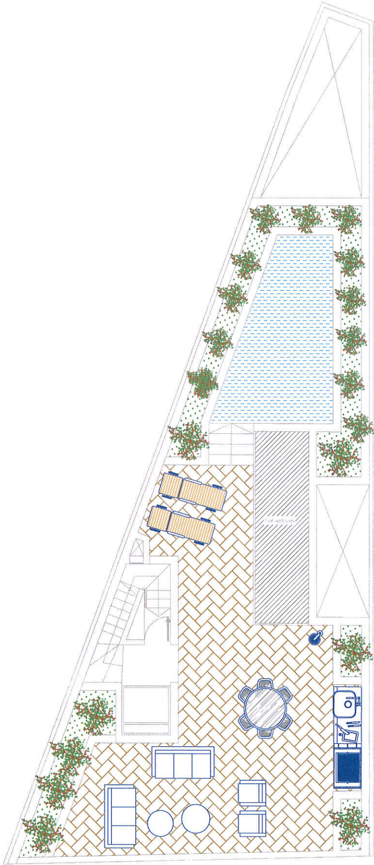
SCALE 1:50 ROOF OVER RECEDED FLOOR
