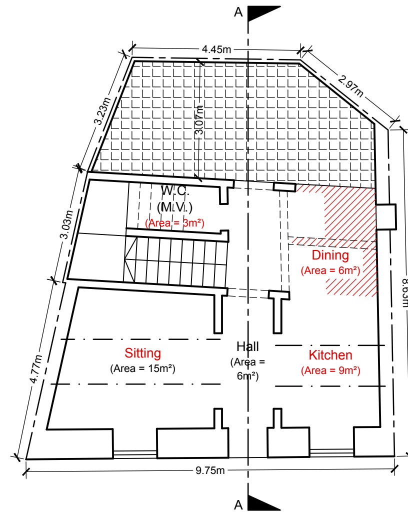
P2 PROPOSED GROUND FLOOR PLAN D1 Floor Area = 86m 2 Scale 1:100
