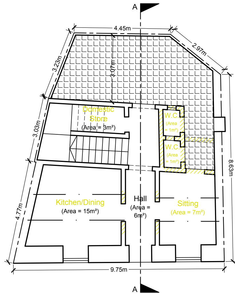
P1 EXISTING GROUND FLOOR PLAN D1 Floor Area = 86m 2 Scale 1:100
