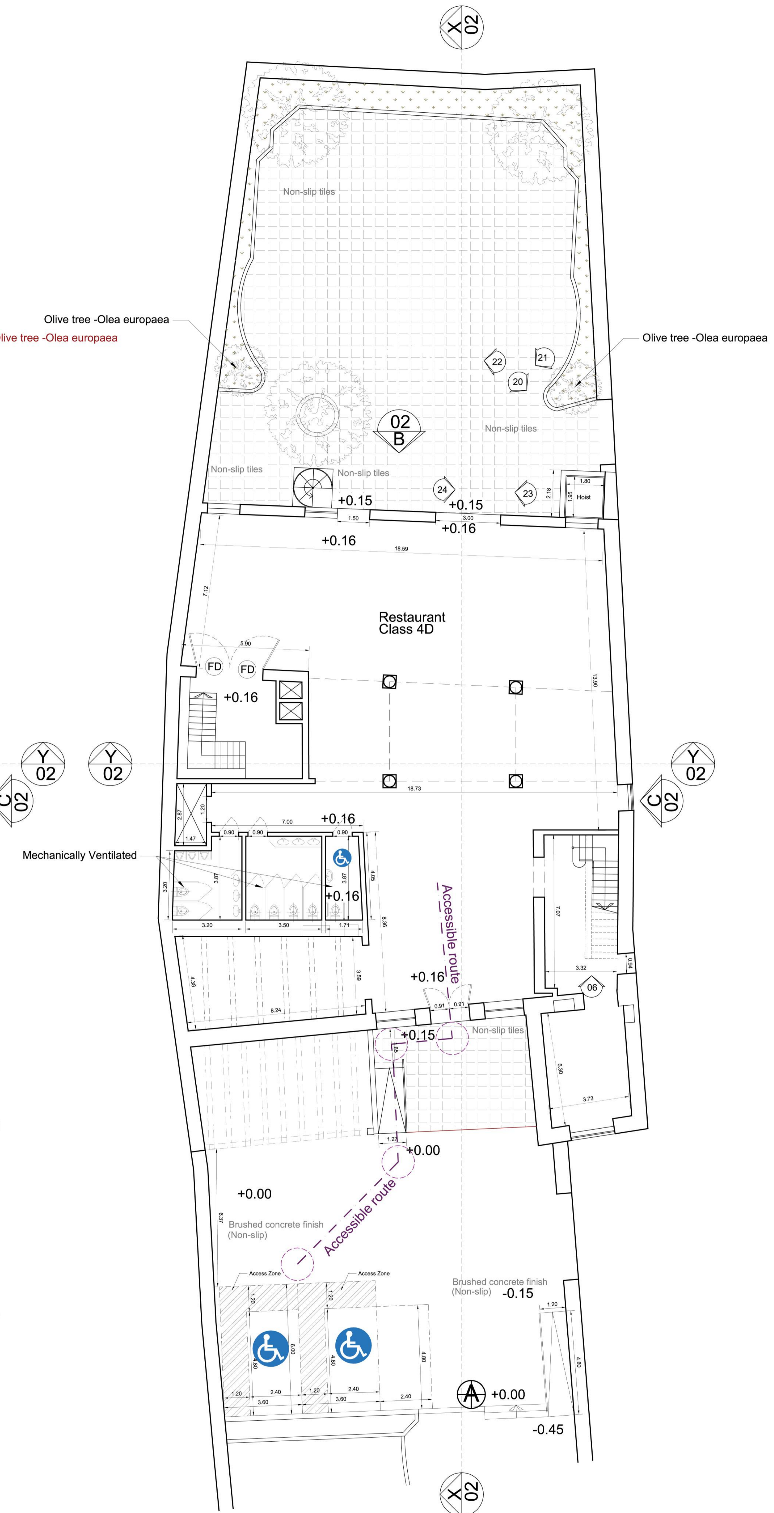
Proposed Ground Floor Part A
