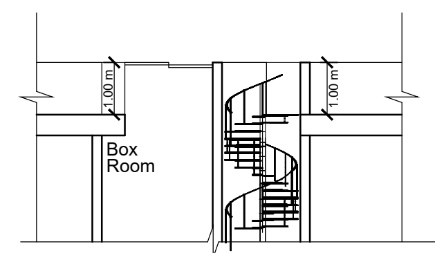
PROPOSED PART SECTION SCALE 1:100
