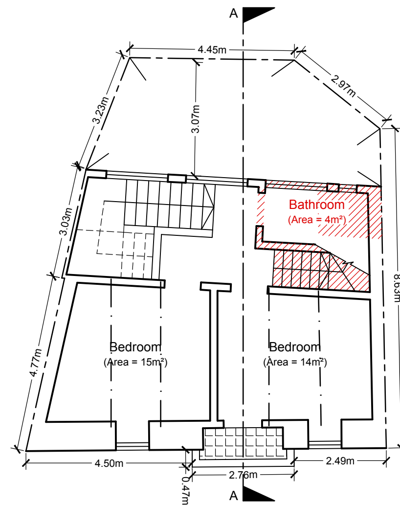
(P4) PROPOSED FIRST FLOOR PLAN (D2) Floor Area = 67m² Scale 1:100
