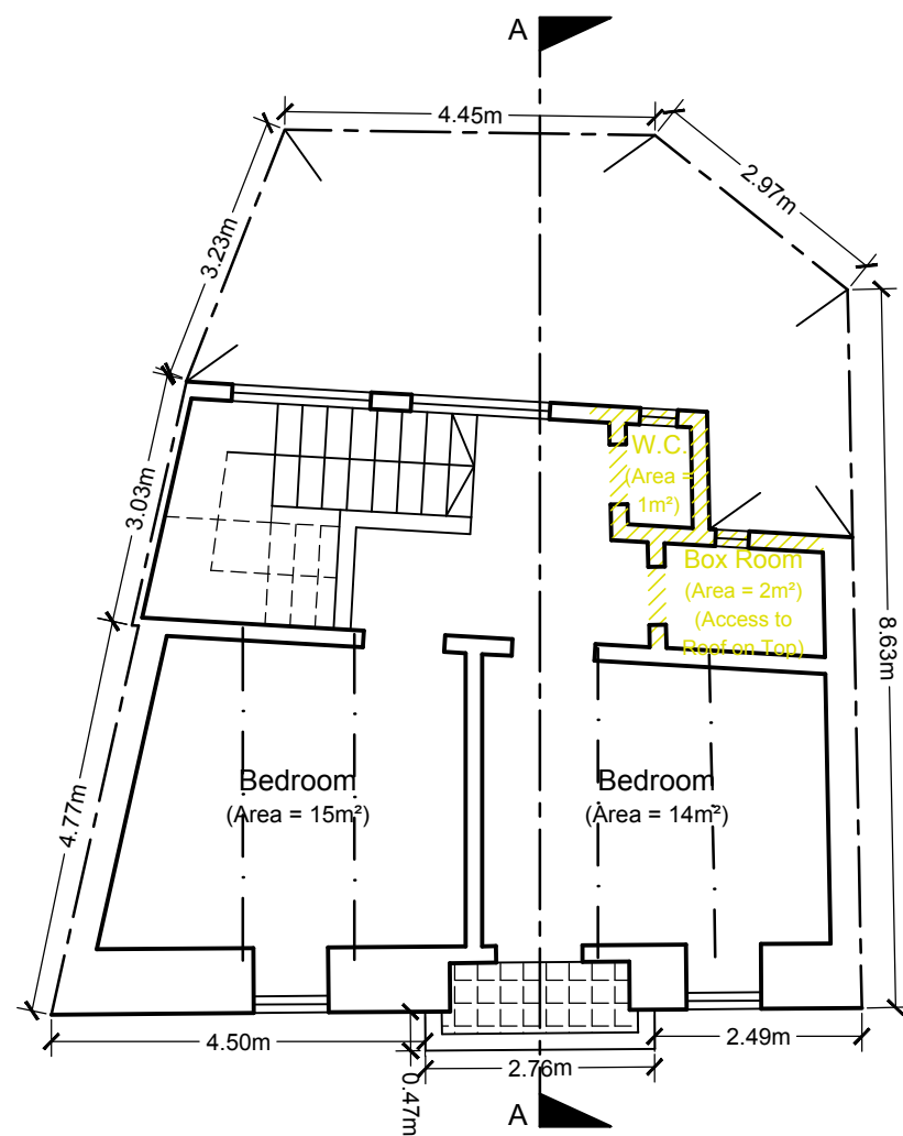
(P3) EXISTING FIRST FLOOR PLAN (D2) Floor Area = 64m² Scale 1:100
