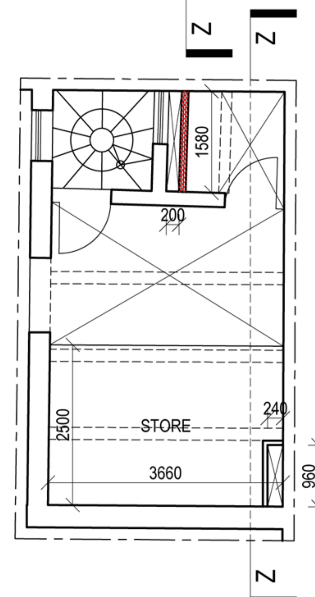
PROPOSED MEZZANIN SCALE 1:100
