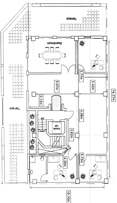
Penthouse Level 5
