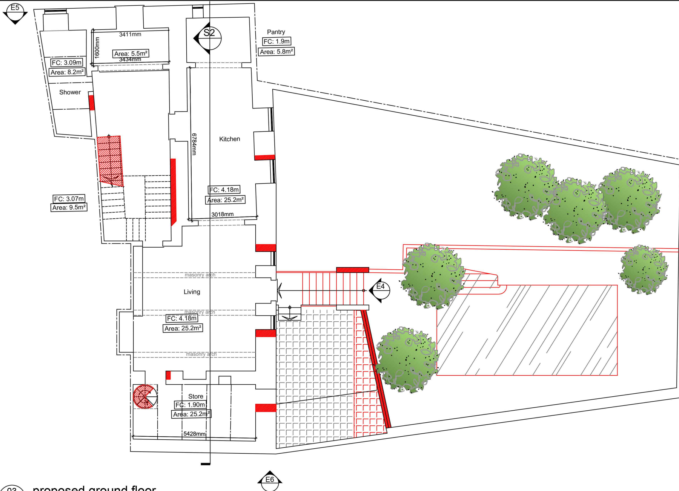
03 proposed ground floor scale 1:100
